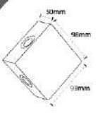
SL 2004 - Round Lens LED : 1x3W, 2x3W, 3x3W, 4x3W Color Temperature : 3000K, 6000K Material: Die-casting Aluminium with Toughened Glass Body Color: Graphite Gray
