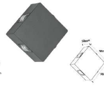
SL 2004 - Square Lens LED : 1x3W, 2x3W, 3x3W, 4x3W Color Temperature : 3000K, 6000K Material: Die-casting Aluminium with Acrylic Square Lens Body Color: Graphite Gray
