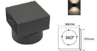
SL 2054 LED : 2X3W Color Temperature : 3000K, 6000K Material: Die-casting Aluminium with Toughened Glass Body Color: Graphite Gray Dimensions : 104 x 101 mm
